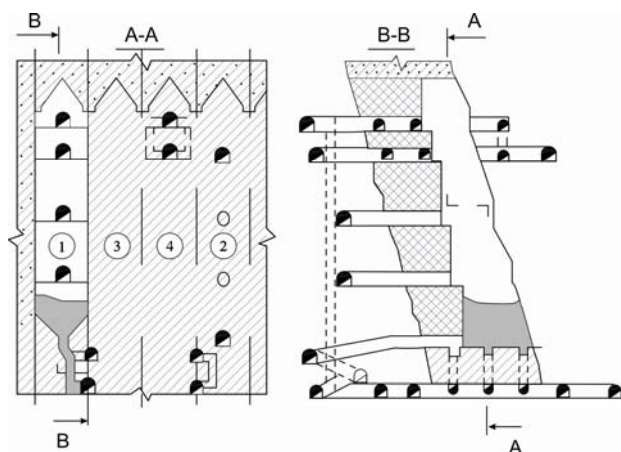
Figure 1. Development system with breaking by sublevel orts with stowing by hardening mixture: 1 – 4 – are the extraction sequence of reserves
