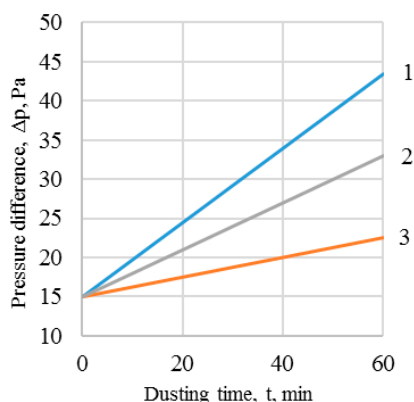
Fig. 6. Change in pressure difference during time in terms of different initial fiber packaging density: 0.05 (1); 0.1 (2); 0.5 (3).
