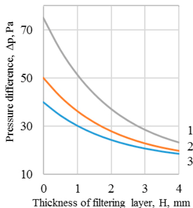
Fig. 5. Curve of changes in pressure difference in terms of filter thickness at different initial concentration of dust particles, \text{mg/m}^3 : 100 (1); 50 (2); 25 (3).
