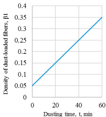
Fig. 7. Change in density of dust-loaded fiber packaging during time in terms of the initial fiber packaging density being 0.05.
