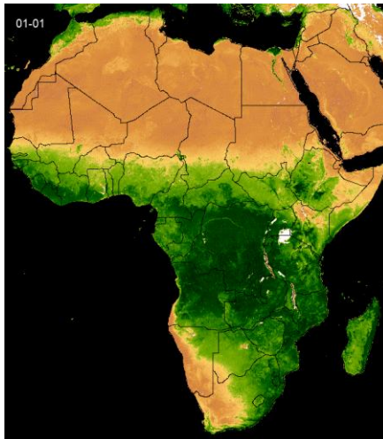
Figure 4 - Visualization NDVI from MODIS period 2020-2025 (Africa)
