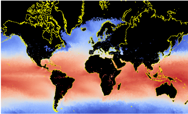
Figure 3 - Visualization Aqua Ocean Color timelapse
