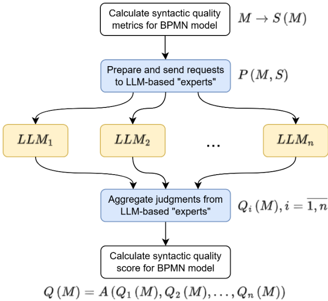
Figure 1 – Conceptual framework of the proposed approach
