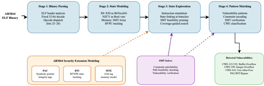
Figure 1 – Four-stage pipeline architecture of the ARM64 digital twin
