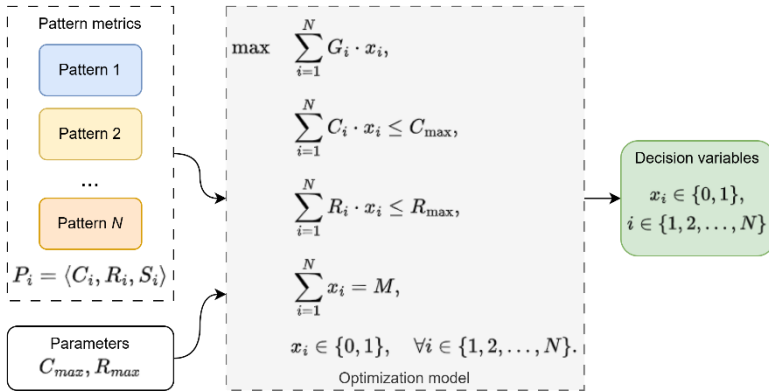
Figure 1 – Conceptual scheme of the proposed approach
