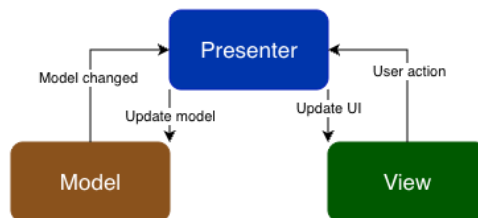
Figure 2 – MVP architecture diagram
