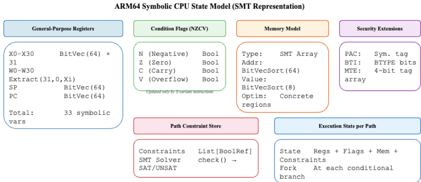
Figure 2 – ARM64 symbolic CPU state model with security extension modeling
