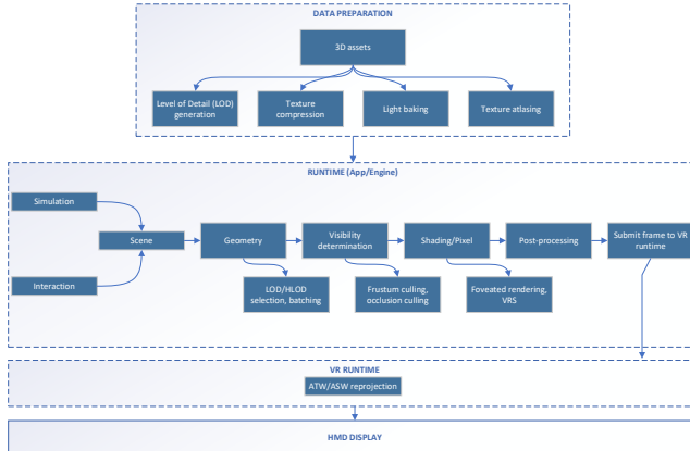
Figure 1 – Structure of the VR visualization pipeline and methods for reducing computational costs and delays
