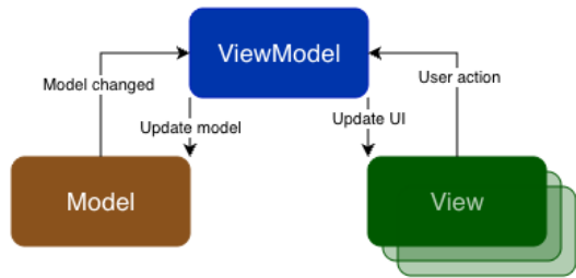
Figure 3 – MVVM architecture diagram
