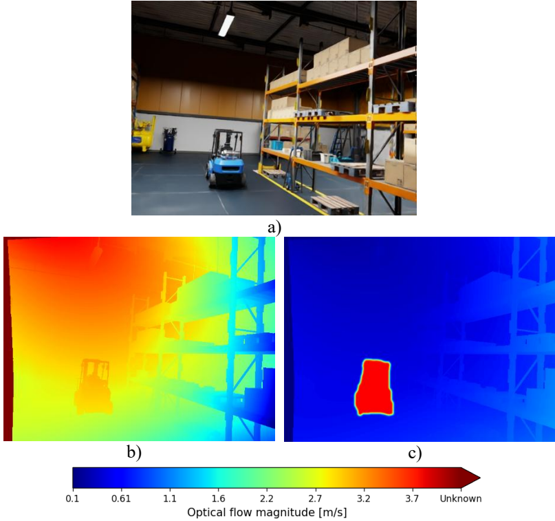
Figure 1 – Residual optical flow pipeline for a single frame in the simulated warehouse: (a) rectified RGB input; (b) estimated dense optical flow; (c) residual flow after ego-motion subtraction.
