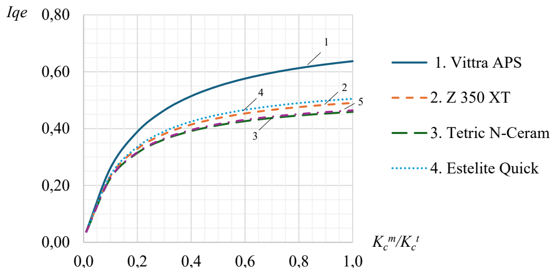
Fig. 3. Dependence of the quality factor on the relative fracture toughness
