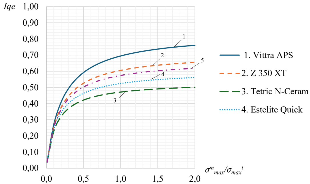
Fig. 2. Dependence of the quality factor on the relative compressive strength
