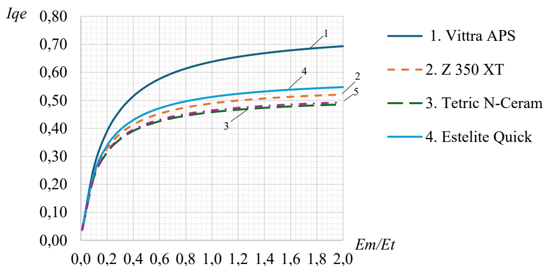
Fig. 1. Dependence of the materials quality factor on the relative elasticity modulus
