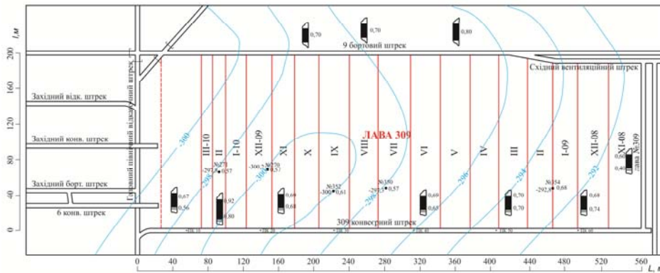
Fig. 1. Copying from the plan of mining works in 309 wallface of the mine "Zarichna" of the SC "L'vivvugillya"
