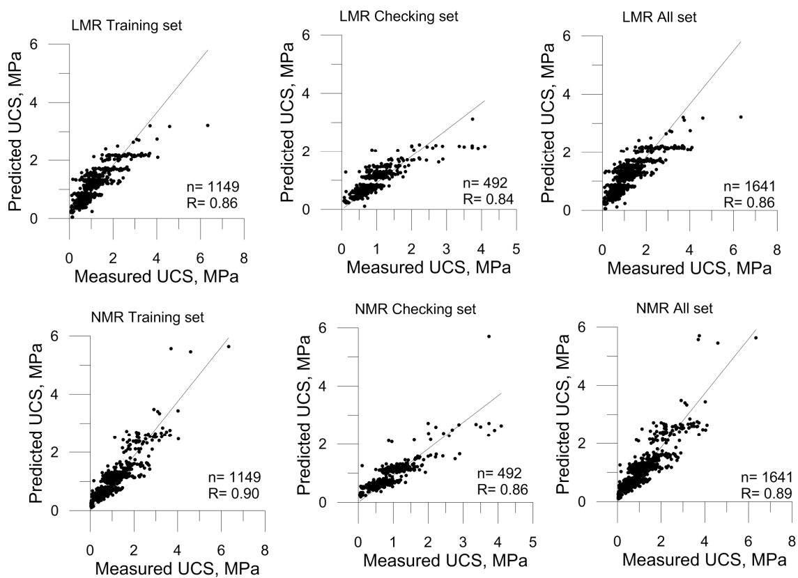
Figure 4. Cross correlation graph for LMR and NMR models
