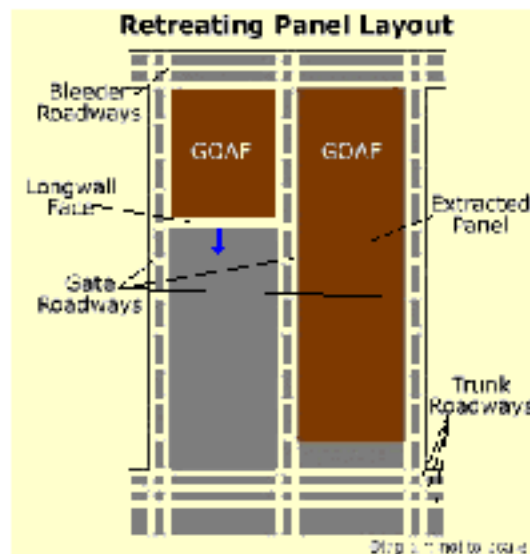
Figure 23. Retreat longwall mining
