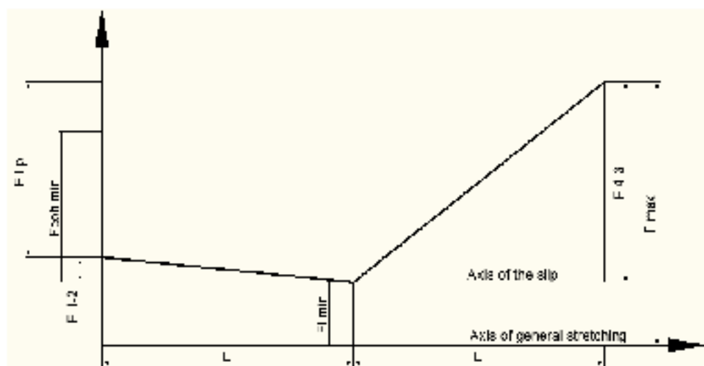
Figure 33. Diagram of belt tension
