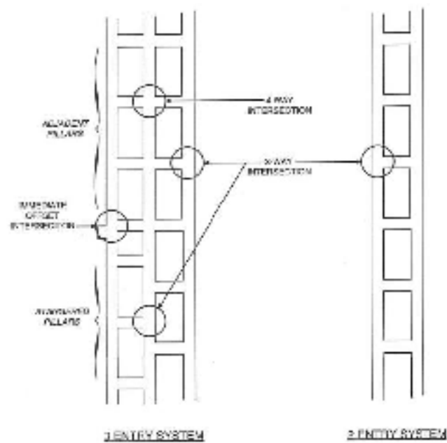
Figure 18. Entry systems
