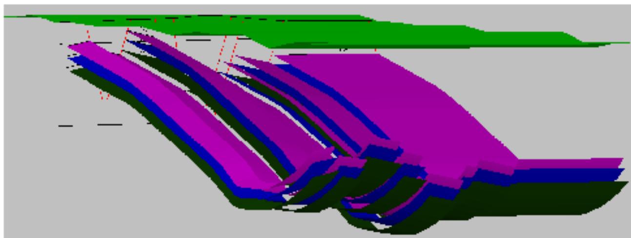
Figure 11. 3D model of the coal seams
