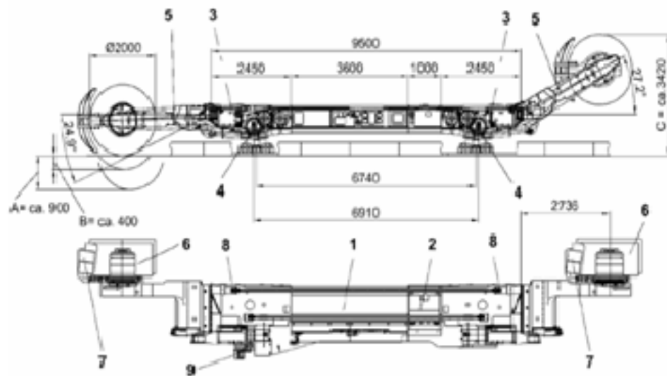
Figure 24. Layout of the shearer loader Eickhoff SI750. 1 – electro unit; 2 – ECP – Box; 3 – electric winch; 4 – wheel housing; 5 – cutting unit; 6 – cutting drum; 7 – plow blade; 8 – tie rod; 9 – line interception.
