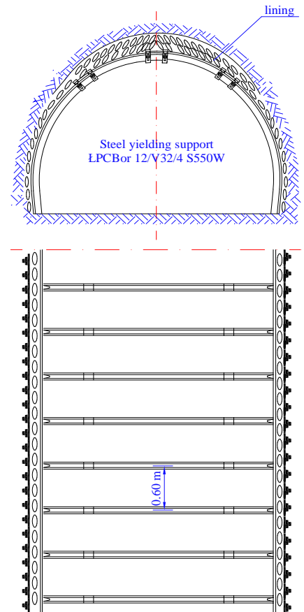
Figure 13. Support scheme in Drift W
