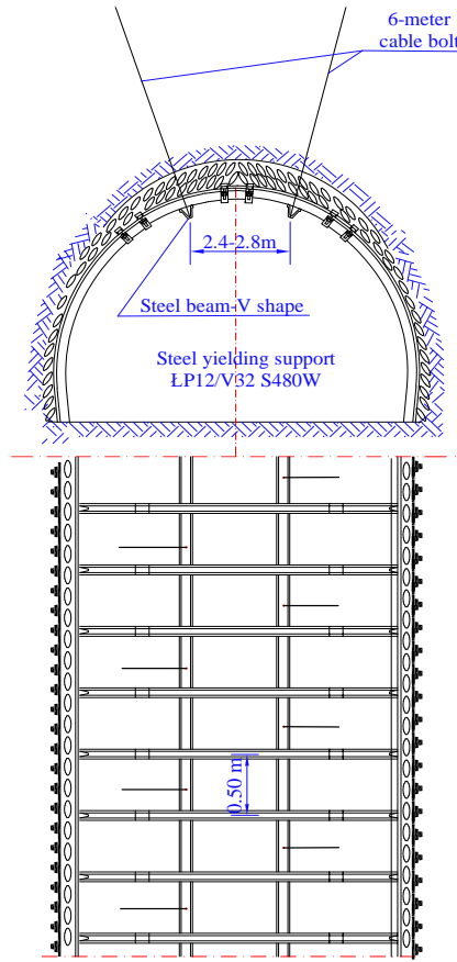
Figure 12. Support scheme in Ventilation drift W-1
