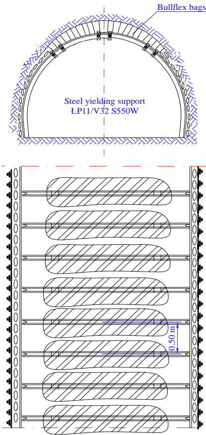
Figure 11. Support scheme in Eastern roadway
