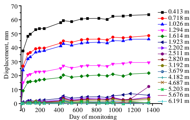
Figure 20. Roof strata displacement in the Eastern roadway
