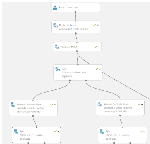
Figure 1 – Processing and separation of input data
