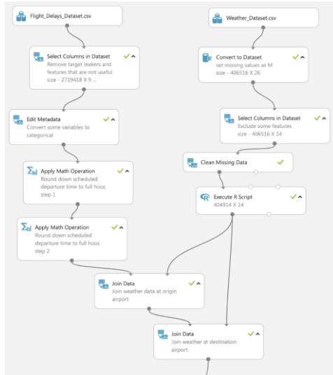
Figure 1 - Implementation of preparation steps with AMS
