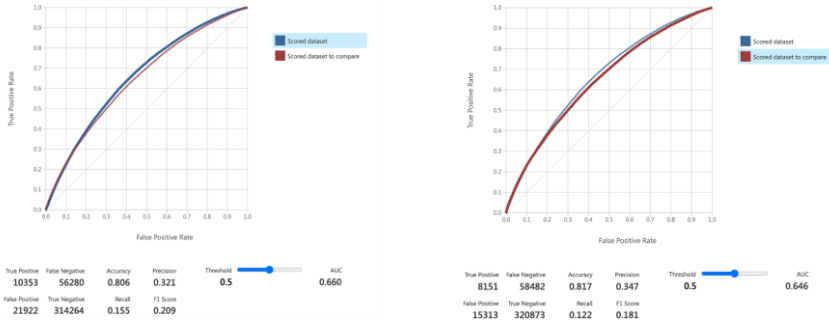
Figure 3 - Data visualizations using ‘two-Class Boosted decision Tree’ and ‘two-Class Logistic regression’ models
